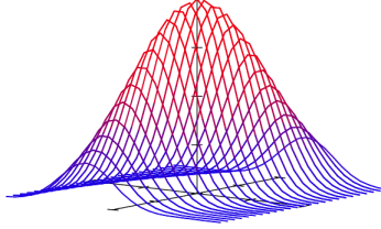
Figure 1: Bivariate normal p.d.f.
