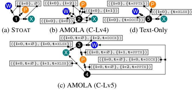
Fig. 3: Partial models. Each circle is a state and each edge is a state transition labeled with a model action. States ②, ③ and ④ are w.r.t. GUI trees of file viewers for DOCX, XLSX and PPTX, respectively. Other states are w.r.t. GUI trees in Fig. 1. Model actions of ListView ( i.e. , w_0^i and w_0^j ) are omitted.
