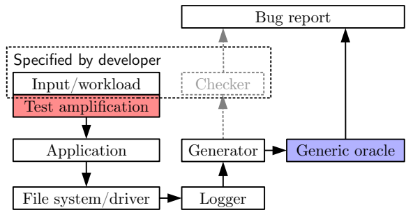
Figure 1: The workflow of crash consistency validation. White background cells denote the workflow of existing work [21, 28, 31]. In comparison, C^3 introduces generic oracle (blue), test amplification (red) and avoids user-specified checker (dashed grey).
