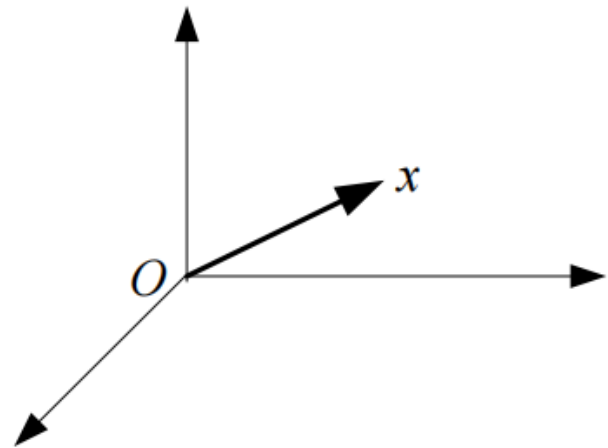
A 3-vector
