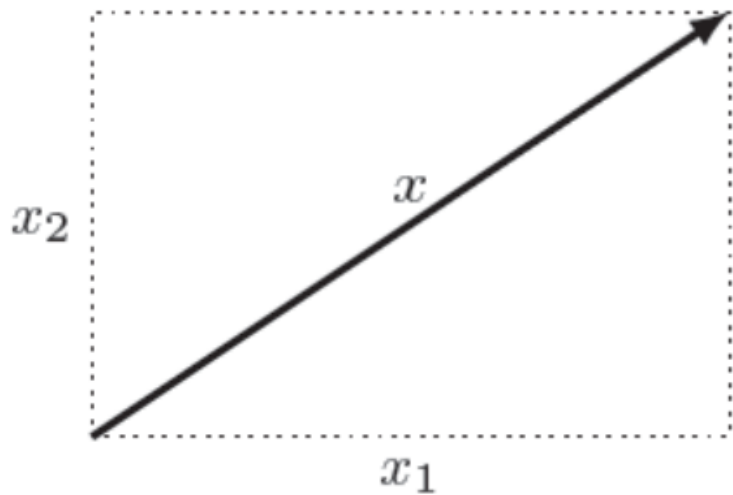
A 2-vector
