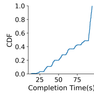
Figure 15: Completion time.
