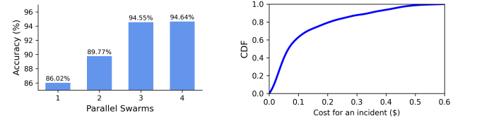
Figure 12: XiHe behaves well with 3 swarms.
