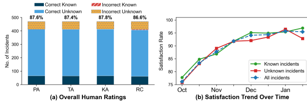
Figure 7: Operators' feedback on XiHE since the latest major OKB update in September 2025.
