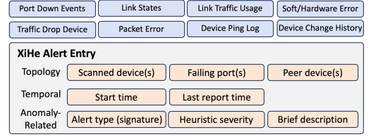
Figure 6: XiProxy normalizes alerts and logs from different sources (blue) to a unified entry (gray).
