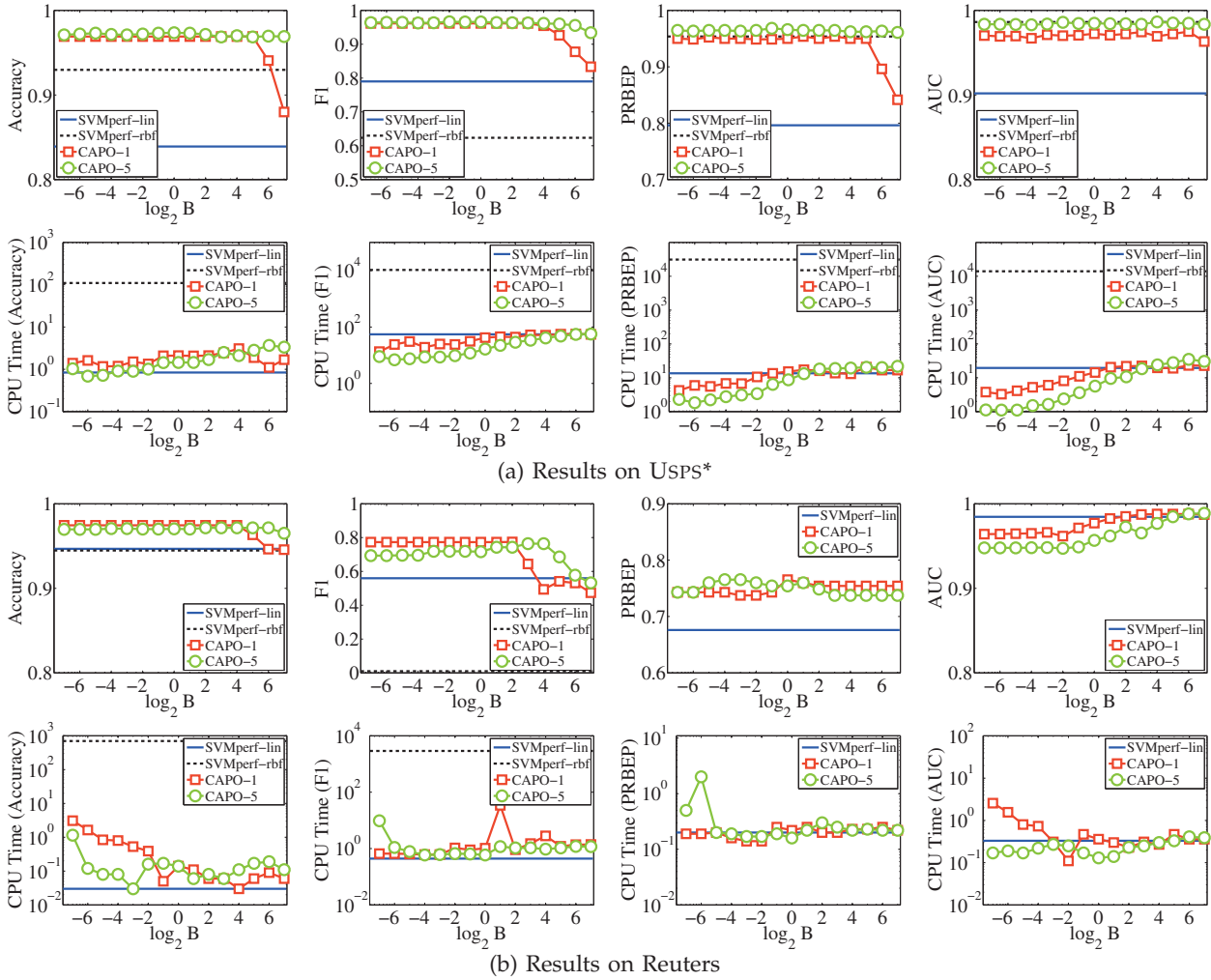
Fig. 4. Performance and CPU time (in seconds) with different B 's: (a) on USPS*, (b) on Reuters. Each subfigure shows performance in the 1st row and corresponding CPU time in the 2nd row.
