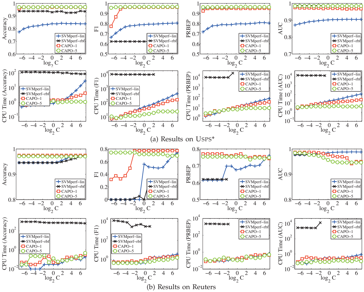
Fig. 3. Performance and CPU time (in seconds) with different C 's, (a) on USPS*; (b) on Reuters. Each subfigure shows performance in the 1st row and corresponding CPU time in the 2nd row.
