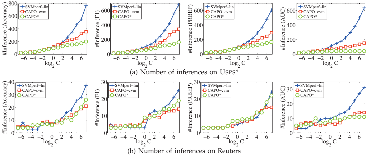
Fig. 1. Number of inferences of the most violated constraints ( \#Inference ) when training SVM_{lin}^{perf} , CAPO_{cvm} and CAPO^* on USPS* and Reuters, where x -axis and y -axis show the C values and \#Inference respectively.
