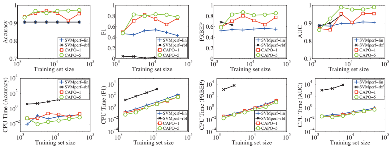
Fig. 5. Performance (1st row) and CPU time (2nd row; in seconds) with different training set sizes on IJCNN.1.
