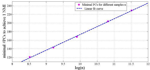
Figure 1. The plot of the smallest number of pairwise constraints (PCs) needed for perfect recovery. The correlation coefficient computed by the linear fit is 0.992, indicating a linear dependence of sample complexity in \log n .
