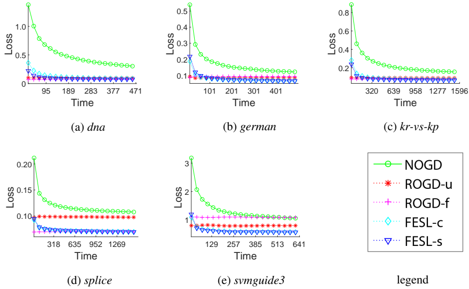
Figure 1: The trend of loss with three baseline methods and the proposed methods on synthetic data. The smaller the cumulative loss, the better.
