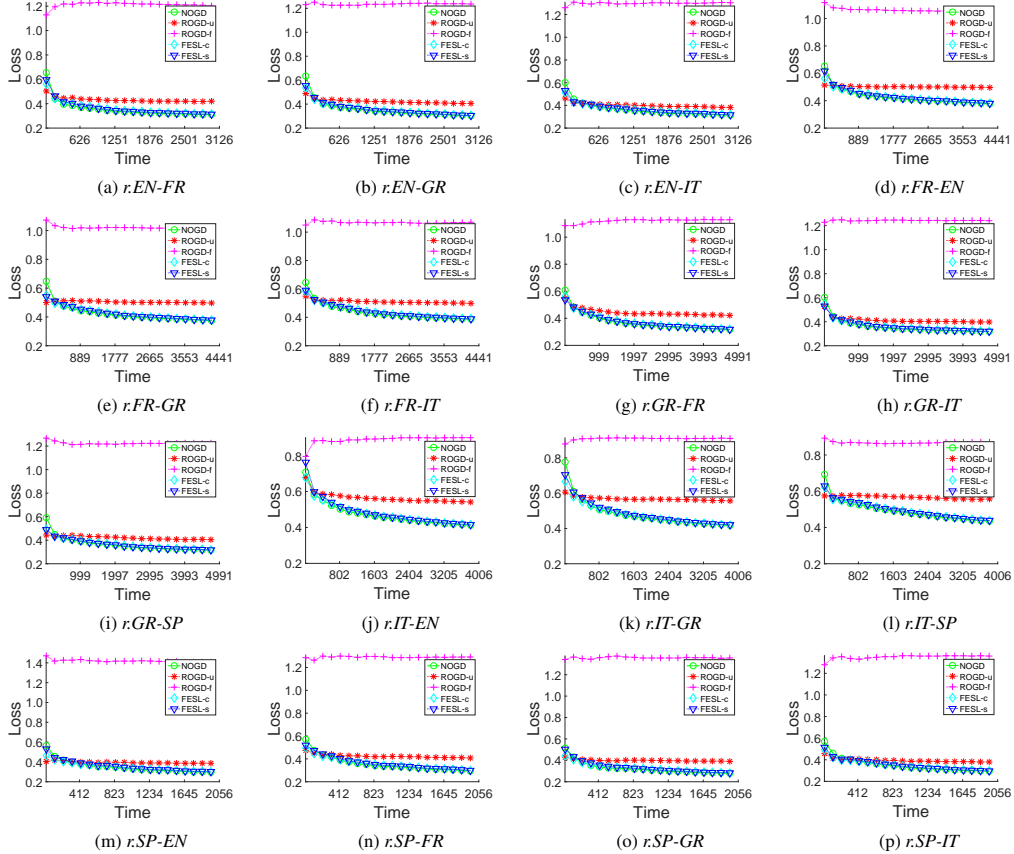
Figure 2: The trend of loss with three baseline methods and the proposed methods on Reuter data. The smaller the cumulative loss is, the better. The average cumulative loss at any time of our methods is smaller than the best of baseline methods.
